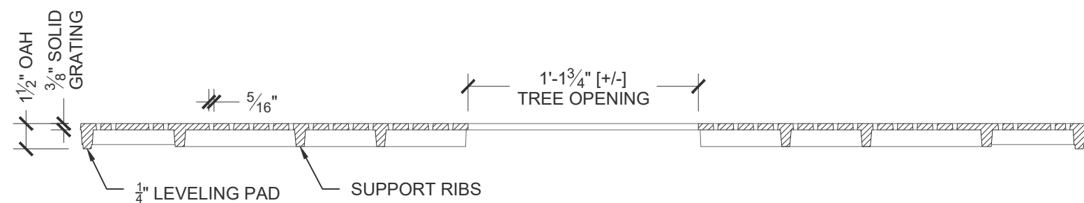
Cross Section Scale: 1 1/2" = 1' 0"
