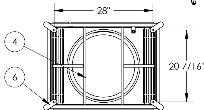
BOTTOM VIEW MOUNTING DETAIL
